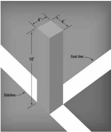
PYLON DETAIL
